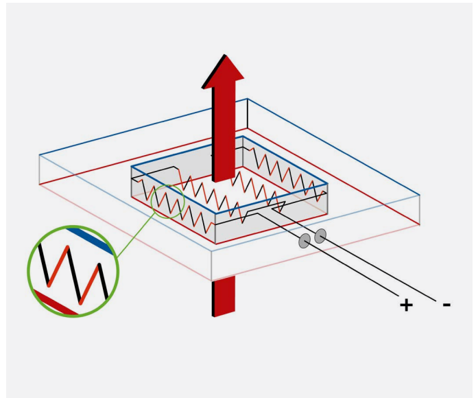
Figure 2 General heat flux sensor principle: the sensor contains a thermopile consisting of an alternating pattern of two metal alloys.
