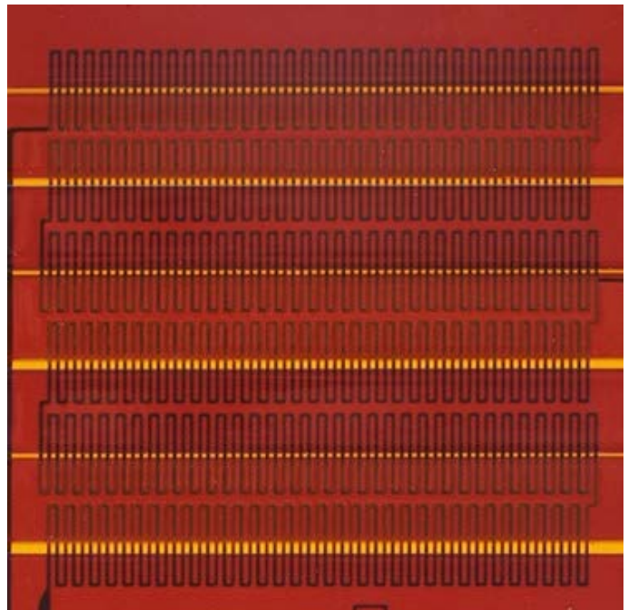
Figure 4 Close-up of a heat flux sensor with a thermopile created using etching and plating technology. A continuous full-metal trace is locally plated and woven through the plastic base material of the sensor.
