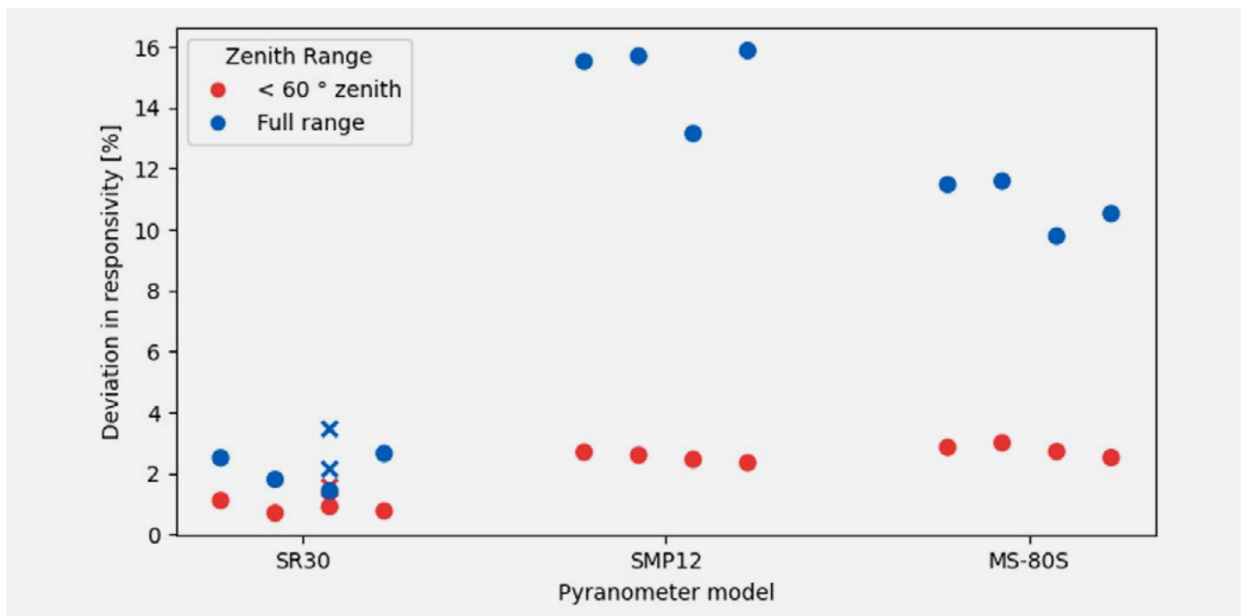
Figure 3 Maximum deviation in responsivity per pyranometer model across four BORCAL datasets. For each model, the data points from left to right correspond to BORCAL reports 2024-02, 2024-03, 2024-04, and 2025 02 respectively. Two additional SR30s are included for BORCAL report 2024-04 (cross markers). Deviations are expressed as percentages relative to the baseline responsivity at 45°, which was used as the reference as recommended by NLR. The zenith range is denoted by color. Clear outliers were excluded from the evaluation of the deviations.
