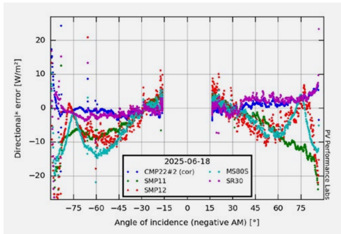
Figure 5 Estimate of the directional* error of different instruments based on NLR data on June 18, 2025. Data points closer to zero correspond to lower errors and therefore better measurements. Negative angles of incidence represent AM measurements and positive angles of incidence represent PM measurements. Source: PV Performance Labs (2025).
