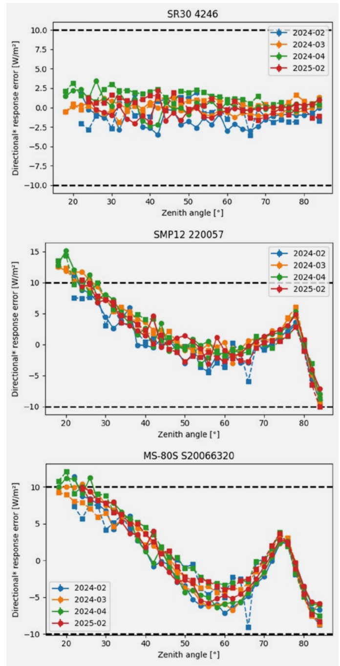
Figure 4 Best-case estimates of the directional* response errors derived from BORCAL responsivity data. Solid lines represent AM measurements and dashed lines PM measurements. Dashed horizontal black lines represent the ISO 9060 Class A limits for directional response.
