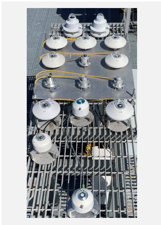
Figure 1 NLR's Global Horizontal West Table with among others Kipp & Zonen SMP12, EKO MS-80S, and Hukx SR30. Image credit: NLR SRRL BMS.
