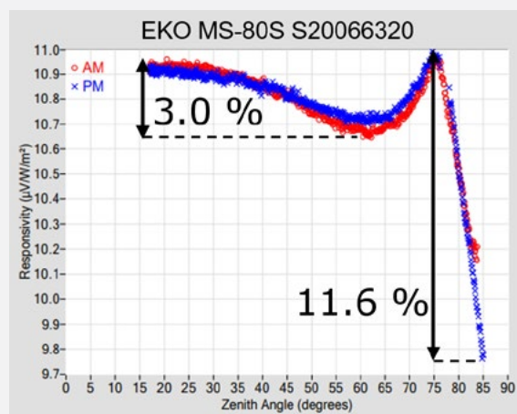
Figure 2 Extract from the NLR 2024-03 BORCAL report showing the responsivity of Hukx's model SR30 with serial number 4246 (p.16), Kipp & Zonen's model SMP12 with serial number 220057 (p.13), and EKO's model MS-80S with serial number S20066320 (p.19) versus zenith angle. The maximum deviation over all angles and over the domain of zenith angles below 60 ° is indicated for every instrument.
