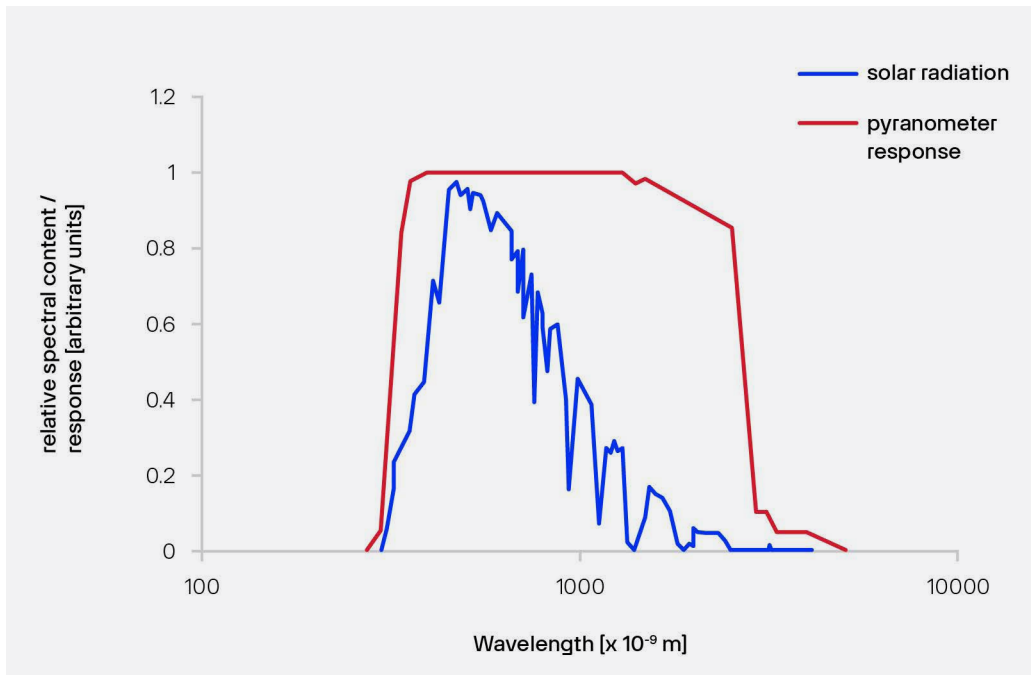
Figure 2.2 Spectral response of the pyranometer compared to the solar spectrum. The pyranometer only cuts off a negligible part of the total solar spectrum.
