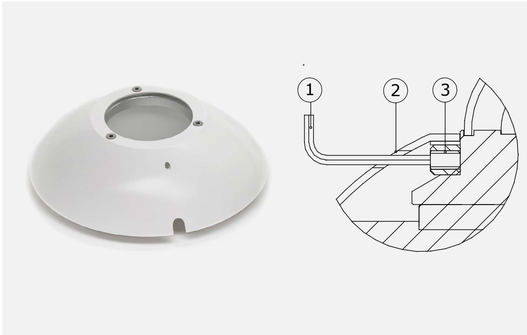
Figure 5.2.1 SCR01 sun screen and its installation and removal: turn the set screw using the hex key and lift off the sun screen to remove. 1. hex key 2. sun screen 3. set screw
