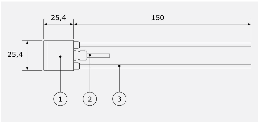
Figure 3.3.1 SGB03-010-02-P150 heat flux sensor with a smooth body, side view dimensions in \times 10^{-3} m.
