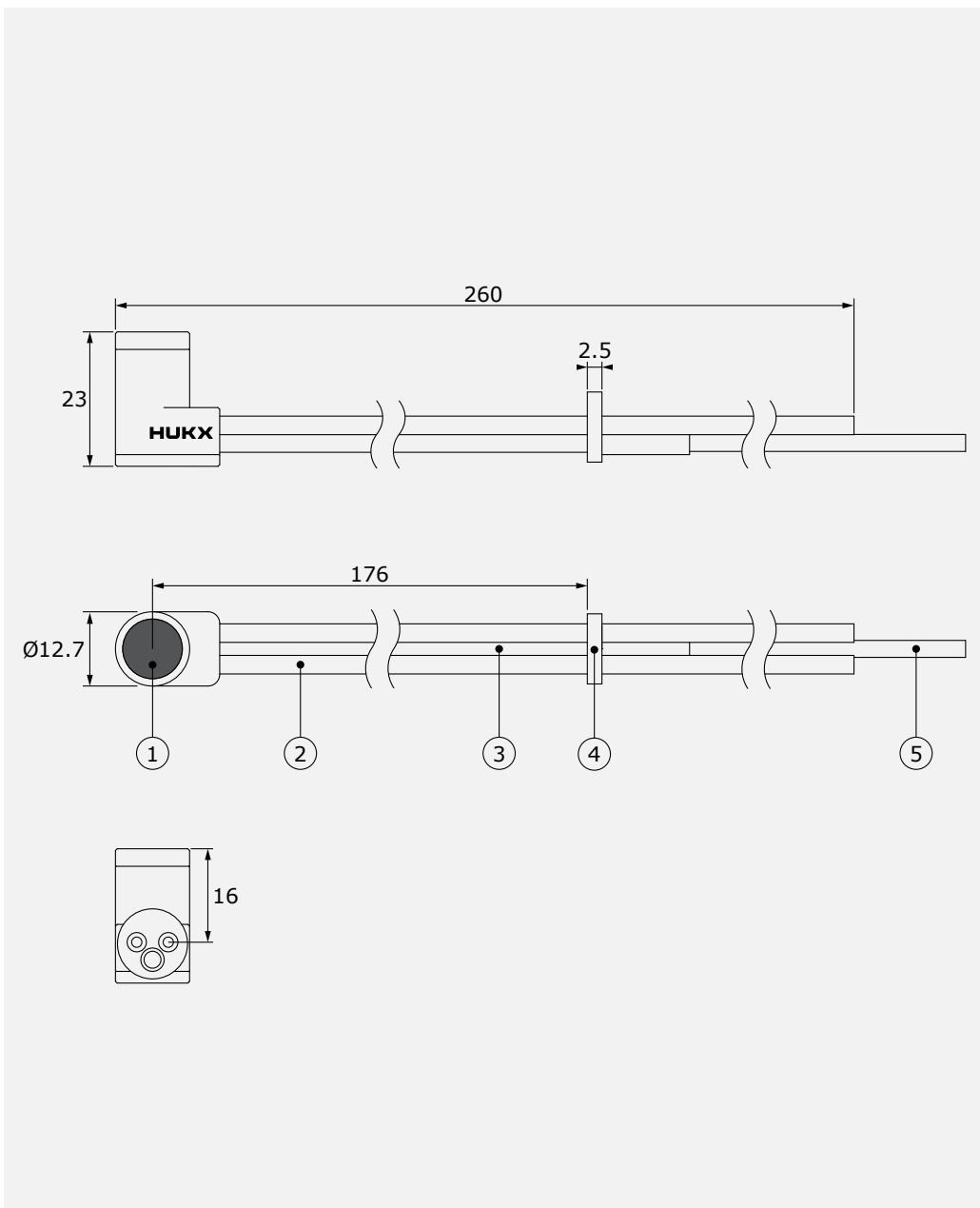
Figure 3.4.1 SGB04 heat flux sensor, dimensions in \times 10^{-3} m. From top to bottom: front view, top view, side view
