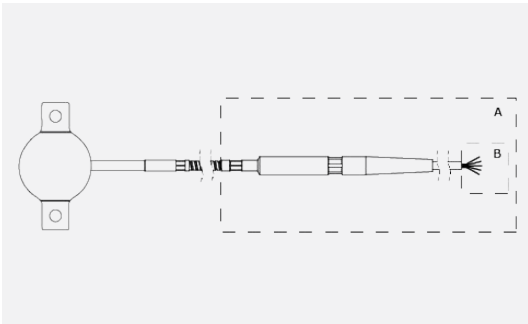
Figure 7.7.1 Only when used with EC type examination certificate (ATEX): IHF01 is certified for use when area A is between -20 and +70 °C, and the cable end (area B) must be provided by the user with an enclosure certified for use in the area of installation.
