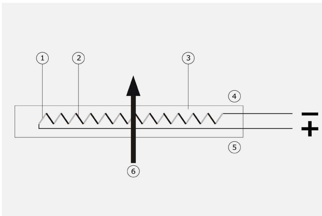
Figure 2.1 The general working principle of a heat flux sensor. The sensor inside IHF02 is a thermopile. A thermopile consists of a number of thermocouples, each consisting of two metal alloys marked 1 and 2, electrically connected in series. A single thermocouple will generate an output voltage that is proportional to the temperature difference between its hot and cold joints. Putting thermocouples in series amplifies the signal. In a heat flux sensor, the hot and cold joints are located at the opposite sensor surfaces 4 and 5. In steady state, the heat flux 6 is a linear function of the temperature difference across the sensor and the average thermal conductivity of the sensor body, 3. The thermopile generates a voltage output proportional to the heat flux through the sensor. The exact sensitivity of the sensor is determined at the manufacturer by calibration and is found on the calibration certificate that is supplied with each sensor.
