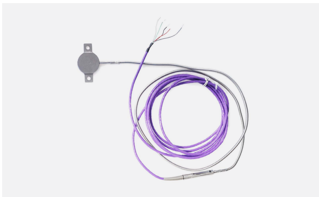
Figure 5.2.1 IHF01 as delivered in its standard configuration.
