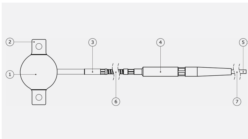
Figure 2.2 IHF01: the heat flux sensor consist of a stainless-steel body (1) which is connected via a rigid stainless steel coupler (3) to a flexible high-temperature metal-sheathed cable with interlocked spiral stainless-steel armor (6). After a transition piece (4), wires are extended using a low-temperature extension cable (7). In the standard configuration, the cable ends in bare wires (5). Two mounting flanges (2) are attached to the body.
