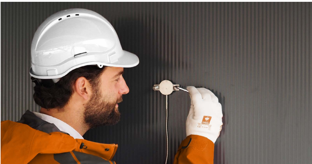
Figure 0.3 IHF01 industrial heat flux sensor mounted on a wall using tack-welded threads and spring-loaded bolts.
