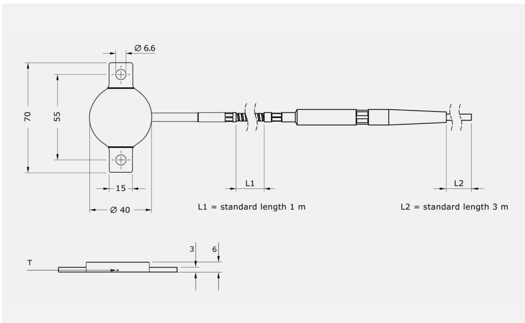
Figure 3.1.1 IHF01 industrial heat flux sensor dimensions in \times 10^{-3} m. T marks the location of the temperature measurement.
