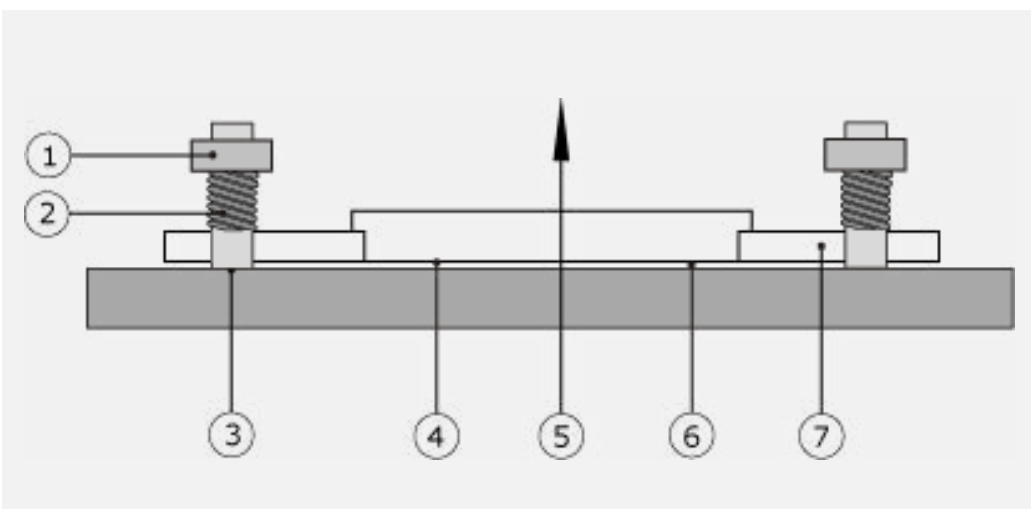
Figure 5.12 Installation of IHF02 on tack-welded threads. 1. M6 bolt 2. spring-loaded M6 thread 3. tack-weld 4. IHF02 side of object to be measured, flush with flanges 5. heat flux generating positive signal 6. for long-term installation, apply high-temperature thread paste or a graphite packing material 7. mounting flange
