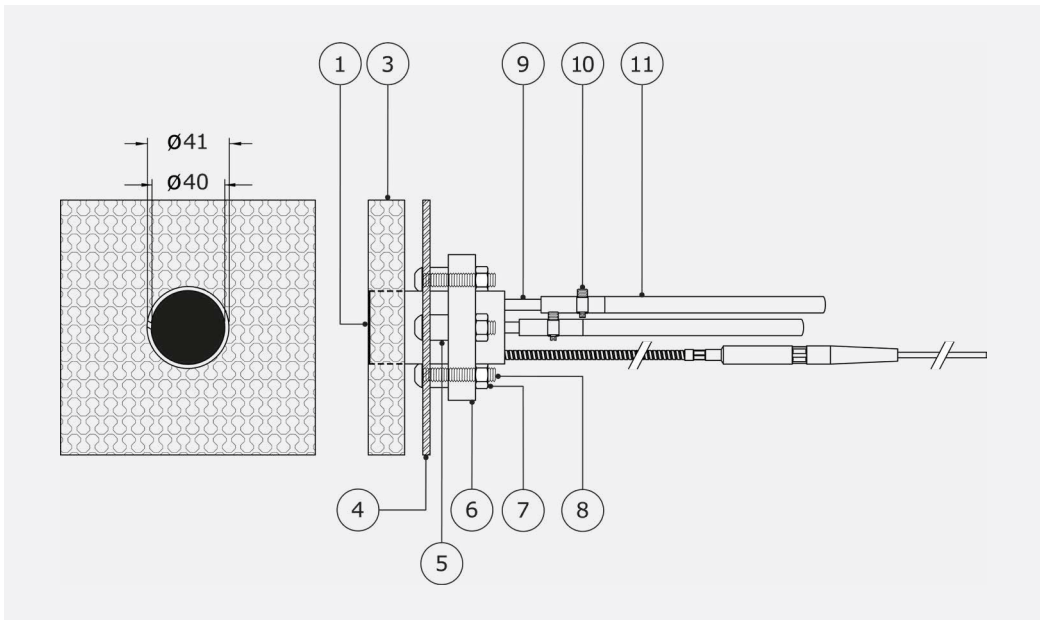
Figure 5.1.2 Recommended installation of HFS01
