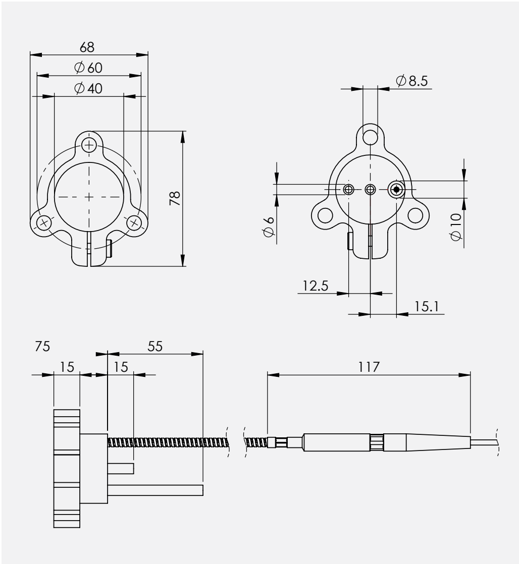
Figure 3.2.1 HFS01 high heat flux sensor dimensions in \times 10^{-3} m.
