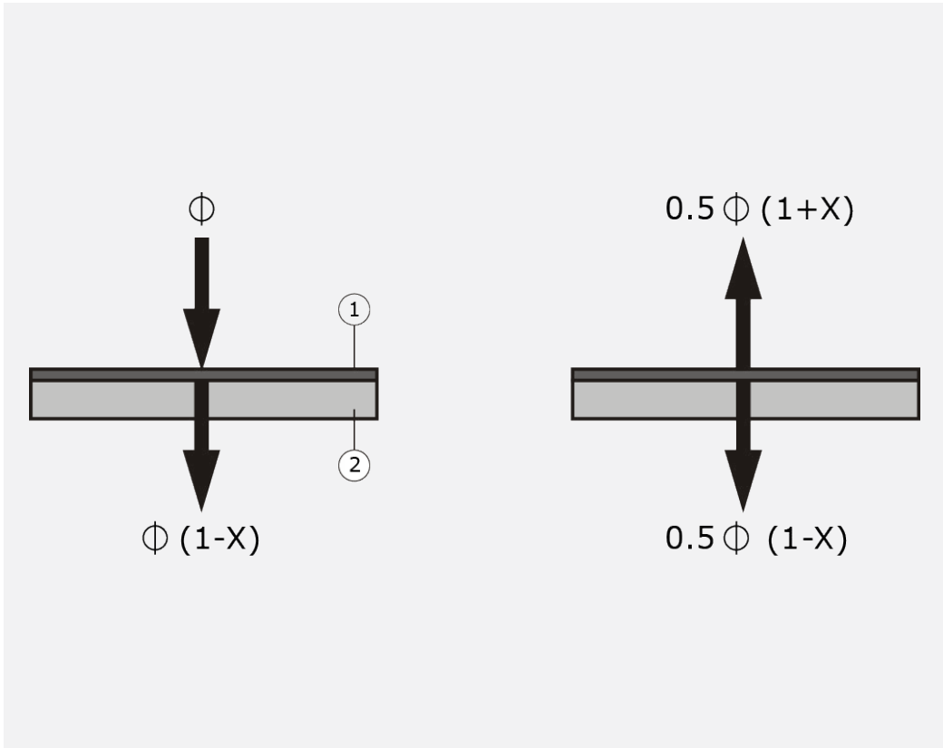
Figure 2.21 Explanation of the self-calibration: on the left, the heat flux sensor (2) measures a soil heat flux \Phi . This flux is subject to a measurement error -X , the deflection error which depends on the thermal conductivity of the soil compared to that of the sensor and its thermal contact to the soil. On the right, during the self-test the film heater (1) is switched on to generate a known electrically generated heat flux. As a first approximation, the division of the total heat flux between downward flux through the sensor and upward flux contains the same (1-X) term that also characterizes the deflection error. The signal level during the self-test, multiplied by 2, is used for self-calibration. The newly measured sensitivity compensates for the deflection error, and also for temperature dependence of the sensitivity and non-stability of the sensor.
