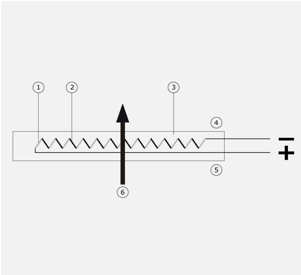
Figure 2.1 The general working principle of a heat flux sensor. The sensor inside HFP01 is a thermopile. A thermopile consists of a number of thermocouples, each consisting of two metal alloys (marked 1 and 2), electrically connected in series. A single thermocouple generates an output voltage that is proportional to the temperature difference between its hot and cold joints. Putting thermocouples in series amplifies the signal. In a heat flux sensor, the hot and cold joints are located at the opposite sensor surfaces (4 and 5). In steady state, the heat flux (6) is a linear function of the temperature difference across the sensor and the average thermal conductivity of the sensor body (3). The thermopile generates a voltage output proportional to the heat flux through the sensor. The exact sensitivity of the sensor is determined at the manufacturer by calibration, and can be found on the product certificate that is supplied with each sensor.
