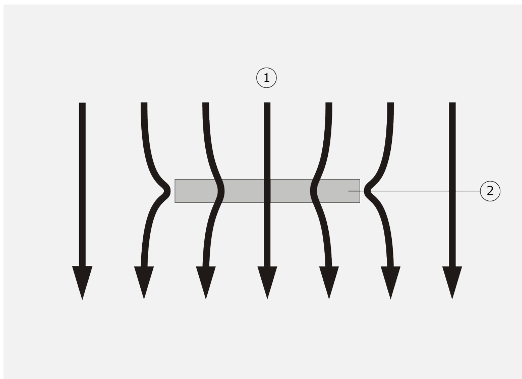
Figure 6.3.3.1 The deflection error. The heat flux (1) is deflected in particular at the edges of the sensor. The measurement will contain an error; the so-called deflection error. The magnitude of this error depends on the thermal conductivity of the environment, sensor thermal conductivity as well as sensor design and contact resistance.
