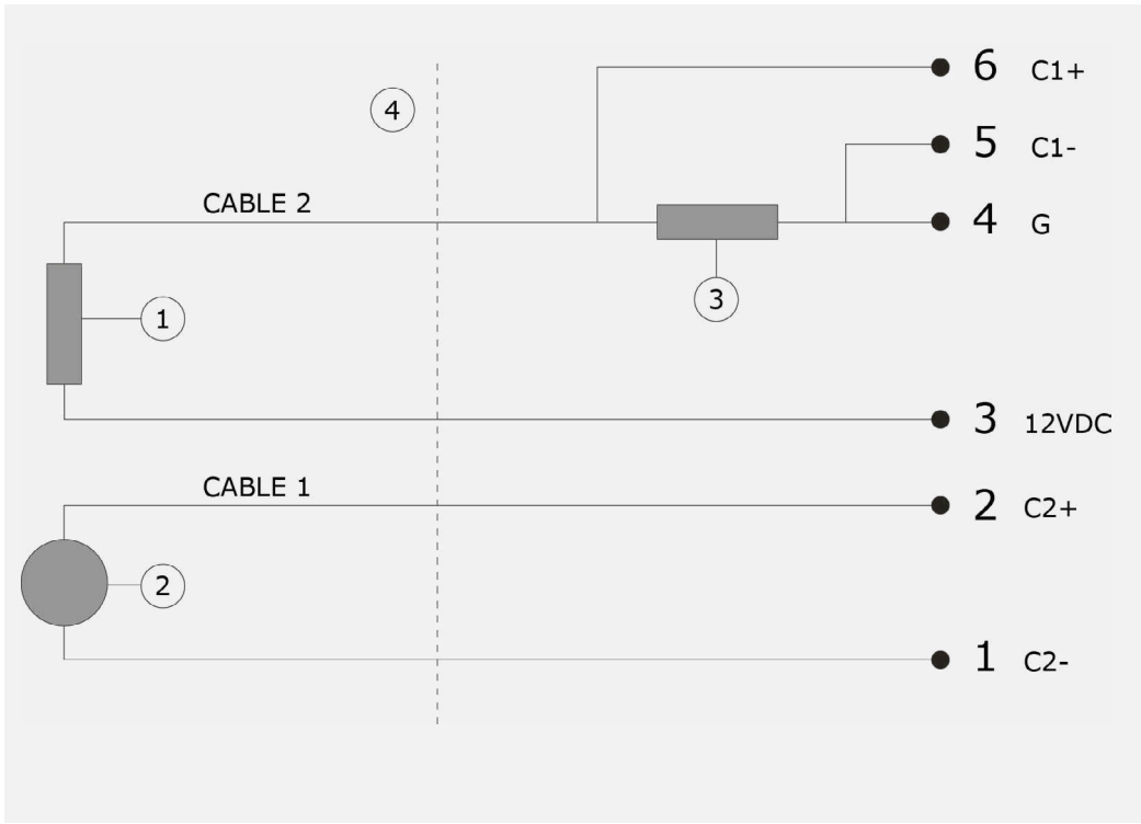
Figure 5.2.1 electrical connection HFP01SC. Dashed line (4) separates between the HFP01SC on the left and the cable and the data logger on the right. Heat flux sensor (2) wires are connected to data logger inputs 1 and 2. Film heater (1) heater wires are connected to the power supply at 3 and 4. The heater current is usually measured using a 10 Ω current sensing resistor (not included with HFP01SC) (3) in series with the heater, and by measuring the voltage across the resistor, at data logger inputs 5 and 6.
