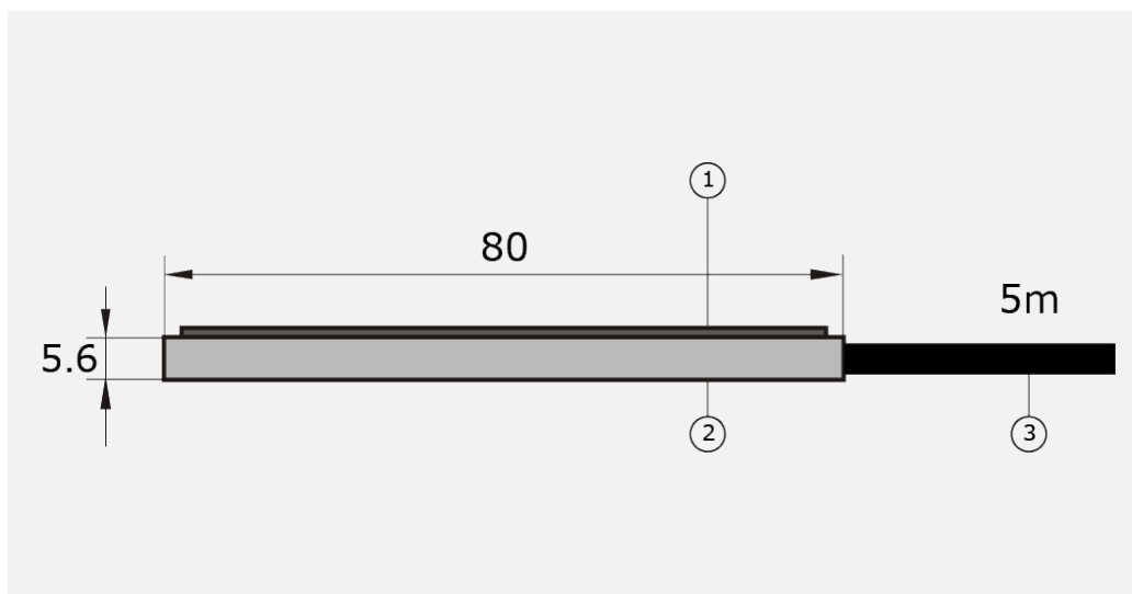
Figure 3.21 HFP01SC heat flux sensor dimensions in \times 10^{-3} m
