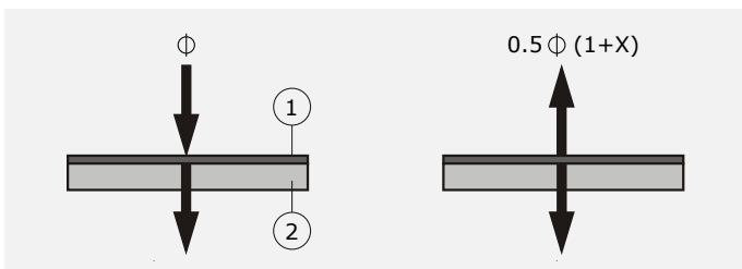
Figure 3 Explanation of the self-calibration: on the left, the heat flux sensor (2) measures a soil heat flux \Phi . This flux is subject to a measurement error - X, the deflection error which depends on the thermal conductivity of the soil compared to that of the sensor and its thermal contact to the soil. On the right, during the self-test the film heater (1) is switched on to generate a known electrically generated heat flux. As a first approximation, the division of the total heat flux between downward flux through the sensor and upward flux contains the same (1-X) term that also characterises the deflection error. The signal level during the self-test, multiplied by 2, is used for self-calibration. The newly measured sensitivity compensates for the deflection error, and also for temperature dependence of the sensitivity and non-stability of the sensor.
