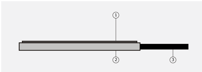
Figure 3 HFP01SC self-calibrating heat flux plate: 1. film heater 2. heat flux sensor plus passive guard, 3. 2 x cable, standard length is 5 m (optionally longer cable).
