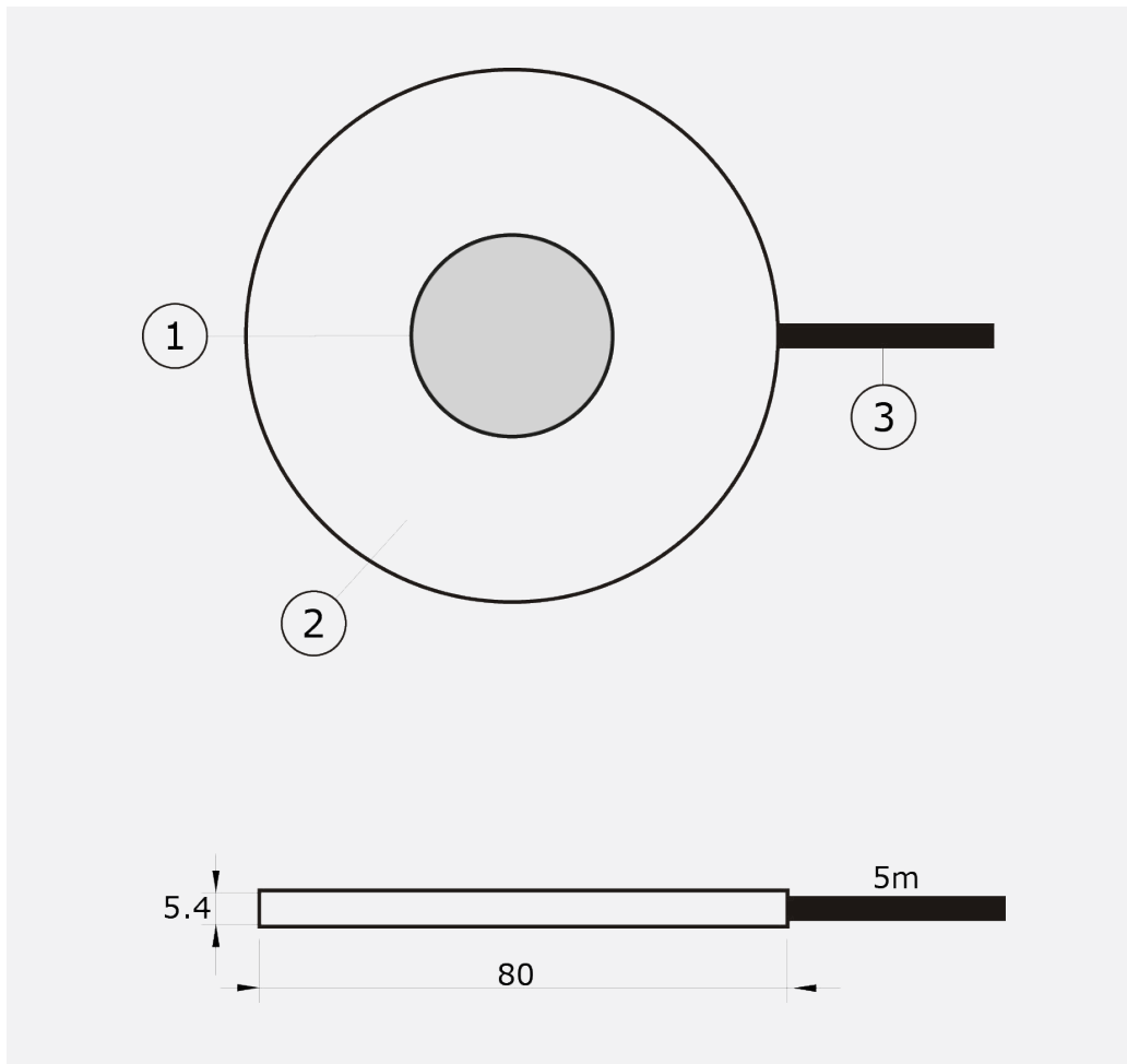
Figure 3.2.1 HFP01 heat flux sensor dimensions in \times 10^{-3} m
