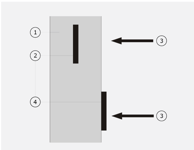
Figure 6.3.3.1 The resistance error: a heat flux sensor (2) increases or decreases the total thermal resistance of the object on which it is mounted (1) or in which it is incorporated. This can either lead to an increase of or decrease of the measured heat flux (3).
