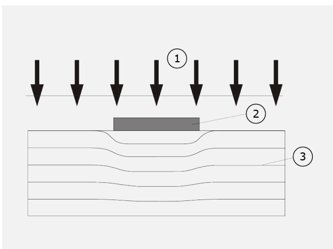
Figure 6.3.3.2 The resistance error: a heat flux sensor (2) increases or decreases the total thermal resistance of the object on which it is mounted or in which it is incorporated. An otherwise uniform flux (1) is locally disturbed. Lines (3) represent isotherms. In this case the measured heat flux is smaller than the actual undisturbed flux, (1).
