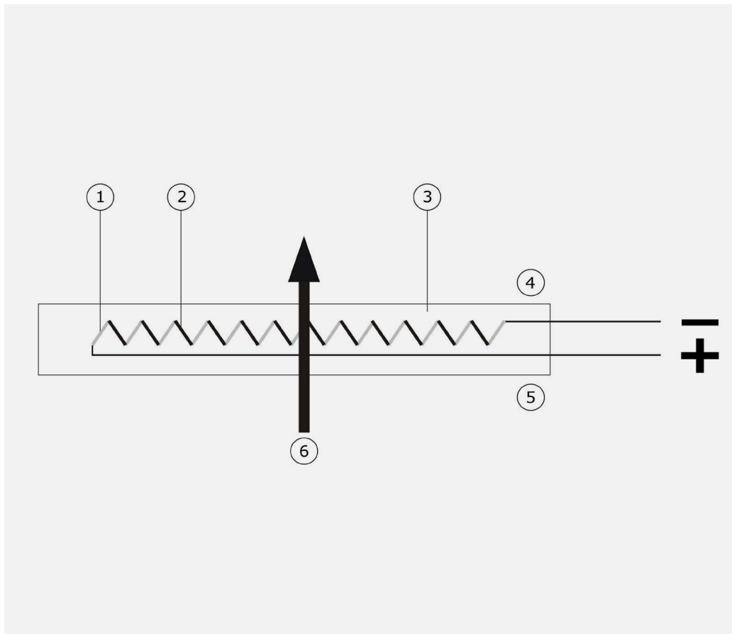
Figure 2.1 The general working principle of a heat flux sensor. The sensor inside HFP01 is a thermopile. A thermopile consists of a number of thermocouples, each consisting of two metal alloys (marked 1 and 2), electrically connected in series. A single thermocouple generates an output voltage that is proportional to the temperature difference between its hot and cold joints. Putting thermocouples in series amplifies the signal. In a heat flux sensor, the hot and cold joints are located at the opposite sensor surfaces (4 and 5). In steady state, the heat flux (6) is a linear function of the temperature difference across the sensor and the average thermal conductivity of the sensor body (3). The thermopile generates a voltage output proportional to the heat flux through the sensor. The exact sensitivity of the sensor is determined at the manufacturer by calibration, and can be found on the product certificate that is supplied with each sensor.
