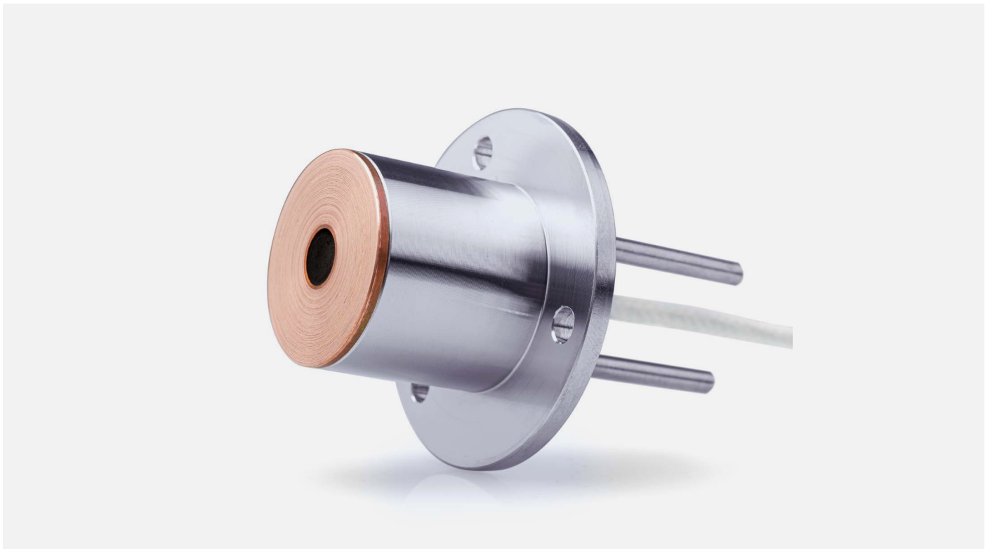
Figure 01 GG01 Gardon gauge water-cooled high heat flux sensor.
