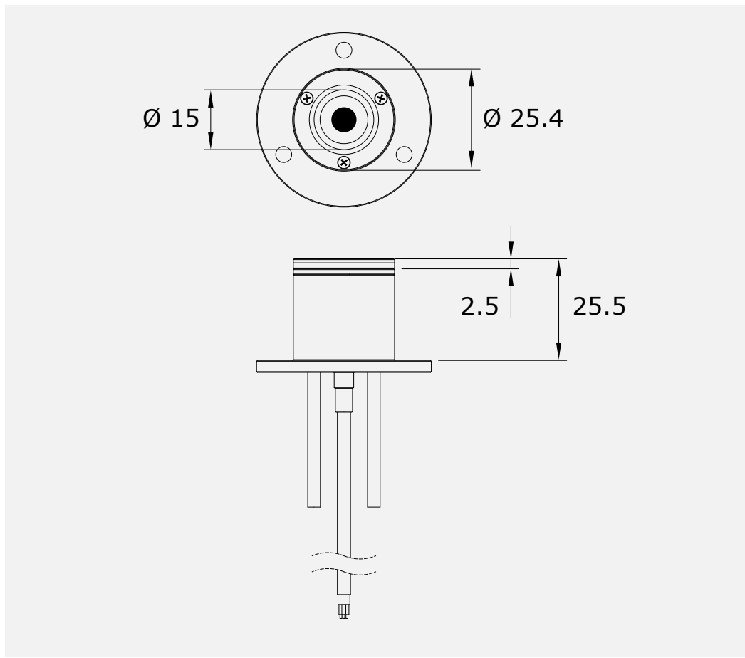
Figure 3.31 GG01 with sapphire window, dimensions in 10^{-3} \text{ m} . The window is added to a standard GG01. GG01s with sapphire window (GG01-250-SW) are custom made, the sapphire window cannot be used on a standard GG01. For other dimensions, see previous section on GG01 dimensions.
