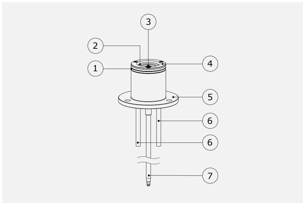
Figure 2.3.2 Overview of GG01-250-SW components: (1) copper housing, (2) sapphire window, (3) thermal sensor with black coating, (4) sapphire window mounting ring, (5) sensor body with flange, (6) water cooling tubes, (7) cable
