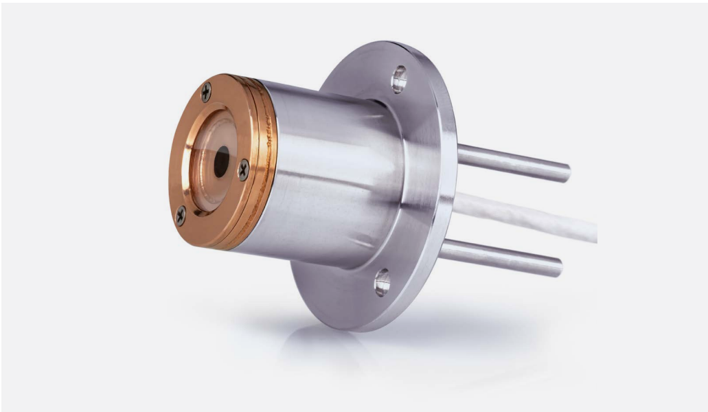
Figure 2.3.1 GG01-250-SW equipped with a sapphire window.
