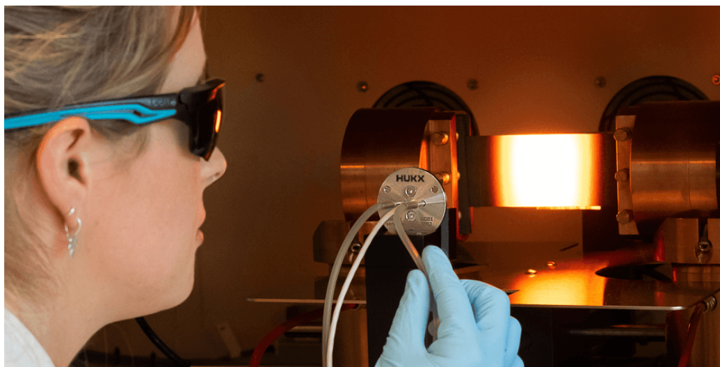
Figure 0.2 GG01 sensor in a high heat flux test cabinet.
