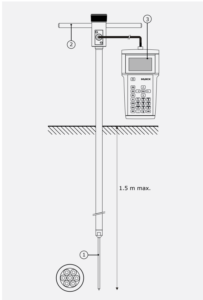
Figure 2 FTN02 system: Mounted at the tip of the lance, LN02 (2), the thermal needle TP09 (1) is inserted into the soil. Users control the measurement using the keyboard and LCD display of CRU02 (3). On the display, the user can monitor the measurement and see the measurement result. After confirmation by the user, results are stored in CRU02's memory. CRU02 contains a rechargeable battery pack for powering the system.
