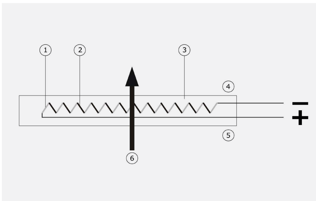
Figure 2.1.1 The general working principle of a heat flux sensor. The sensor inside FHF06 is a thermopile. A thermopile consists of a number of thermocouples, each consisting of two metal alloys (marked 1 and 2), electrically connected in series. A single thermocouple generates an output voltage that is proportional to the temperature difference between its hot and cold joints. Putting thermocouples in series amplifies the signal. In a heat flux sensor, the hot and cold joints are located at the opposite sensor surfaces (4 and 5). In a steady state, the heat flux (6) is a linear function of the temperature difference across the sensor and the average thermal conductivity of the sensor body (3). The thermopile generates a voltage output proportional to the heat flux through the sensor. The exact sensitivity of the sensor is determined at the manufacturer by calibration, and can be found on the product certificate that is supplied with each sensor.
