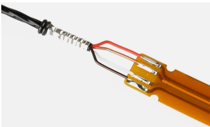
Figure 7.2.2 FHF06 sensor foil with soldered wires.
