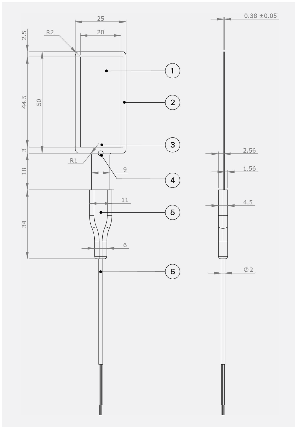
Figure 3.2.1 Model FHF06 with dimensions in \times 10^{-3} m.
