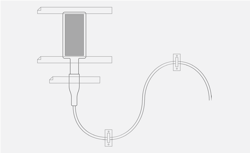
Figure 5.2.1 Installation of model FHF06 using tape to fixate the sensor and the connection block. Extra strain relief on the cable is provided using cable tie mounts equipped with double-sided tape as an adhesive. As indicated in Table 5.1.1, tapes used for mounting the sensor are preferably taped over the passive guard area and not on the sensing area (the latter indicated by grey shading in Figure 5.1.1). Please note the dot is visible in this image; this indicates that we are viewing the frontside and that the other side, the backside, is attached to the object on which the sensor is mounted, as explained in Chapter 2.
