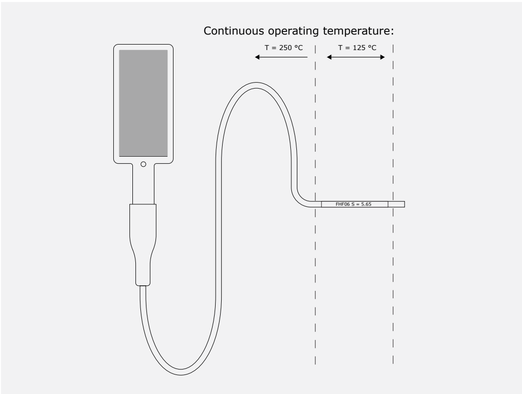
Figure 5.2.2 The label at the end of the cable showing serial number and sensitivity can handle only temperatures up to 125 °C. The sensor, cable and connection block have a continuous operating temperature up to 250 °C.
