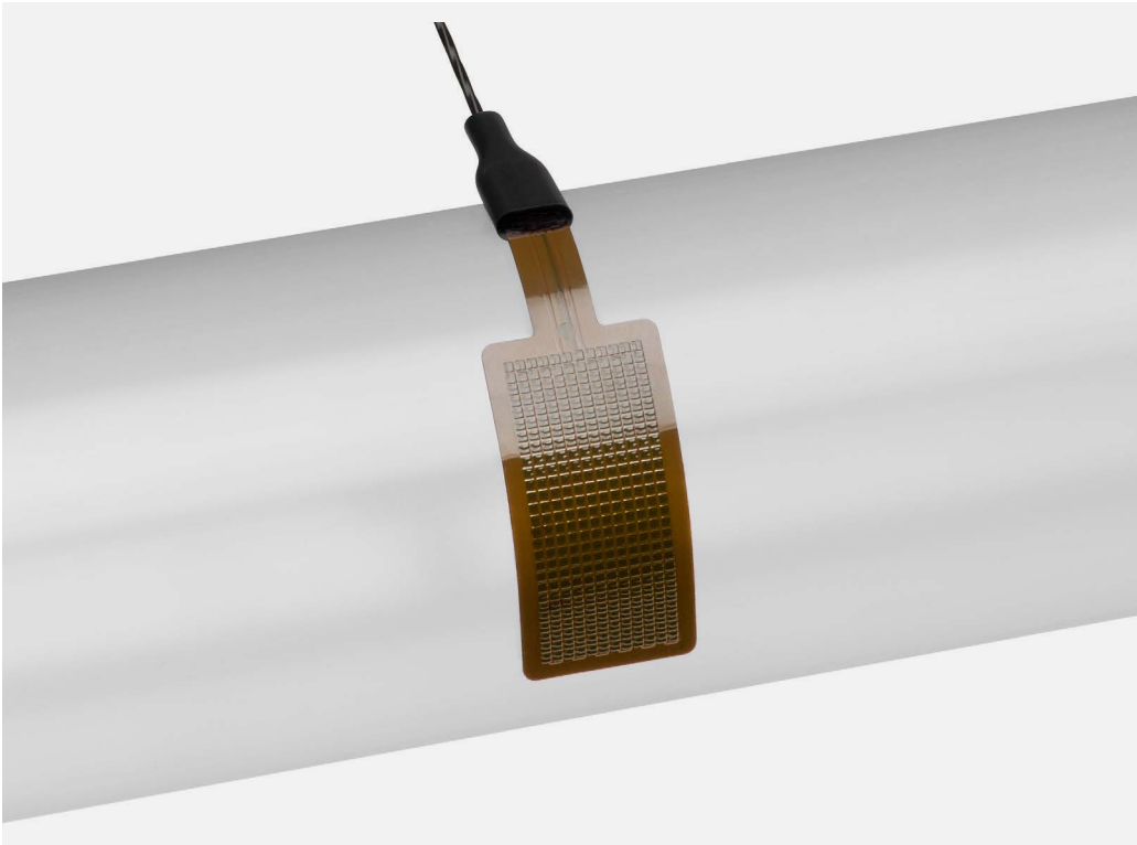
Figure 5.3.1 Bending of model FHF06 foil heat flux sensor, in this image on a pipe.
