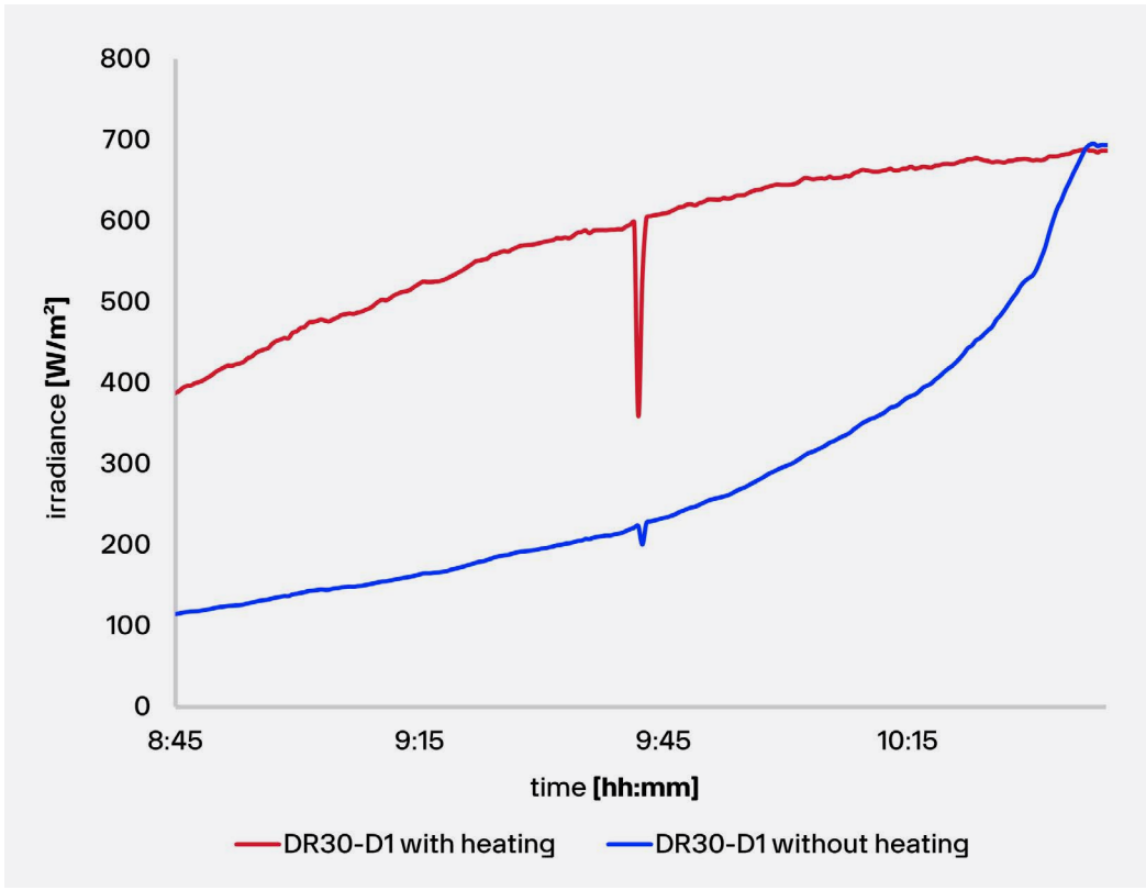
Figure 0.6 Comparison of the measured data with and without heating on a typical winter morning. The unheated DR30 has dew on its front window and strongly underestimates the incoming irradiance. At around 10:30 the dew evaporates. Real measured data from Delft, the Netherlands.
