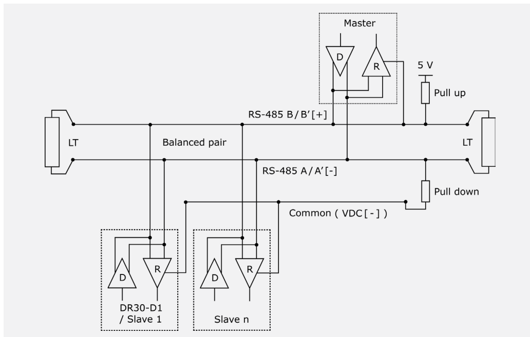
Figure 6.6.1 Typical topology of a two-wire RS-485 network, figure adapted from: Modbus over serial line specification and implementation guide V1.02 ( www.modbus.org ). The power supply is not shown in this figure.
