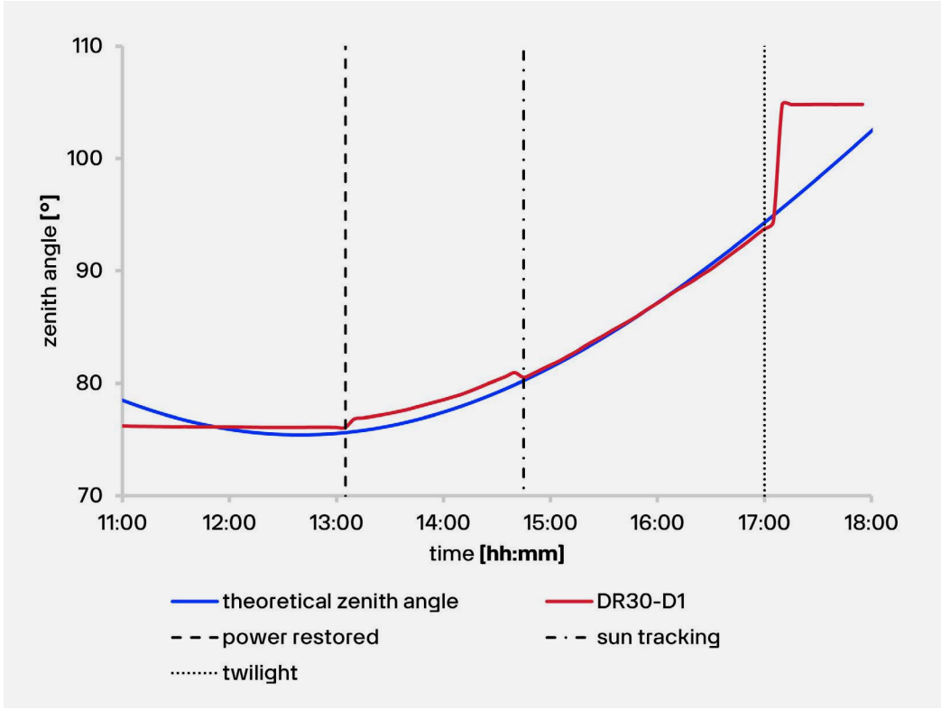
Figure 0.7 Example of use of the DR30 tilt sensor for tracker performance monitoring: the red line is the output of the DR30 tilt sensor, the blue line the theoretical zenith angle. There is a power failure before 13:00, at that time power is restored. Tracking between 13:00 and 15:00 is under cloudy conditions, based on GPS information only and slightly off. Tracking from 15:00 onwards is under sunny conditions and based on the tracker's sun sensor. The tracker moves to its rest position shortly after 17:00. Real measured data from Delft, the Netherlands.
