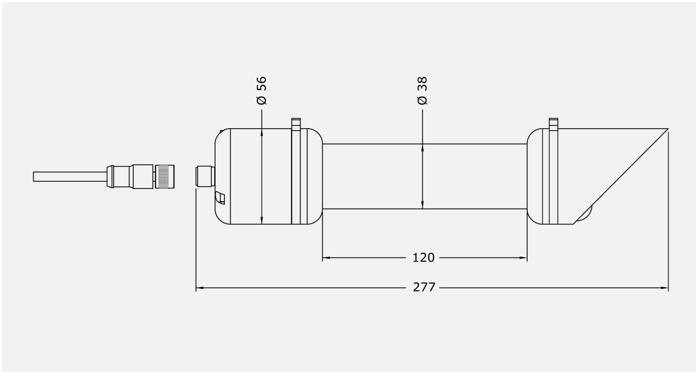
Figure 3.2.1 Dimensions of DR30 in \times 10^{-3} m.
