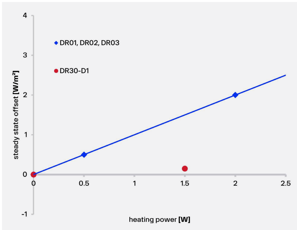
Figure 0.5 The offset of DR30 when heating is much improved relative to the older DR01, DR02 and DR03 models. DR30 has a 1.5 W heater and produces a negligible offset. The older models had offsets of the order of 2 W/m 2 at the same heating levels. In addition, the temperature of the front window of DR30 is 4 times higher than that of the older models, at the same heating power.
