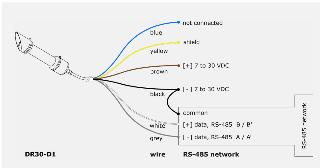
Figure 7.9.1 Connecting DR30 to a typical RS-485 network.
