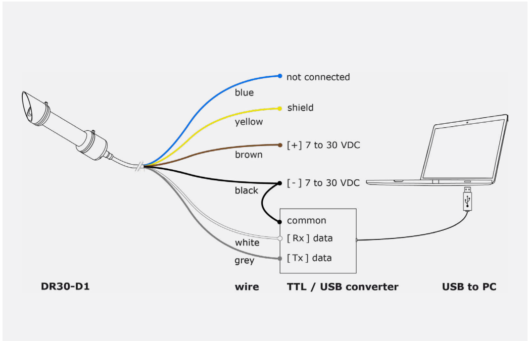
Figure 6.7.1 Connecting DR30 to an RS-485 to USB converter and a PC.
