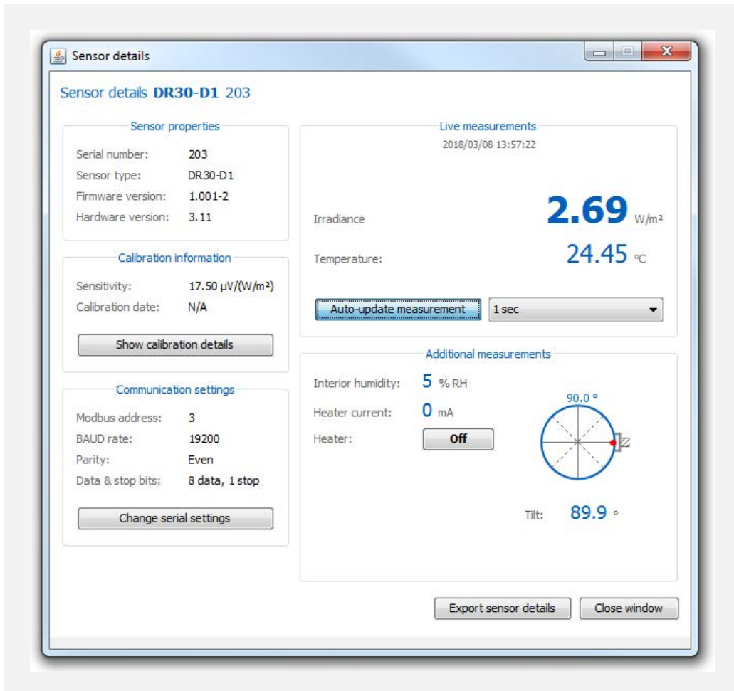
Figure 7.5.1 Sensor details window in the Sensor Manager.
