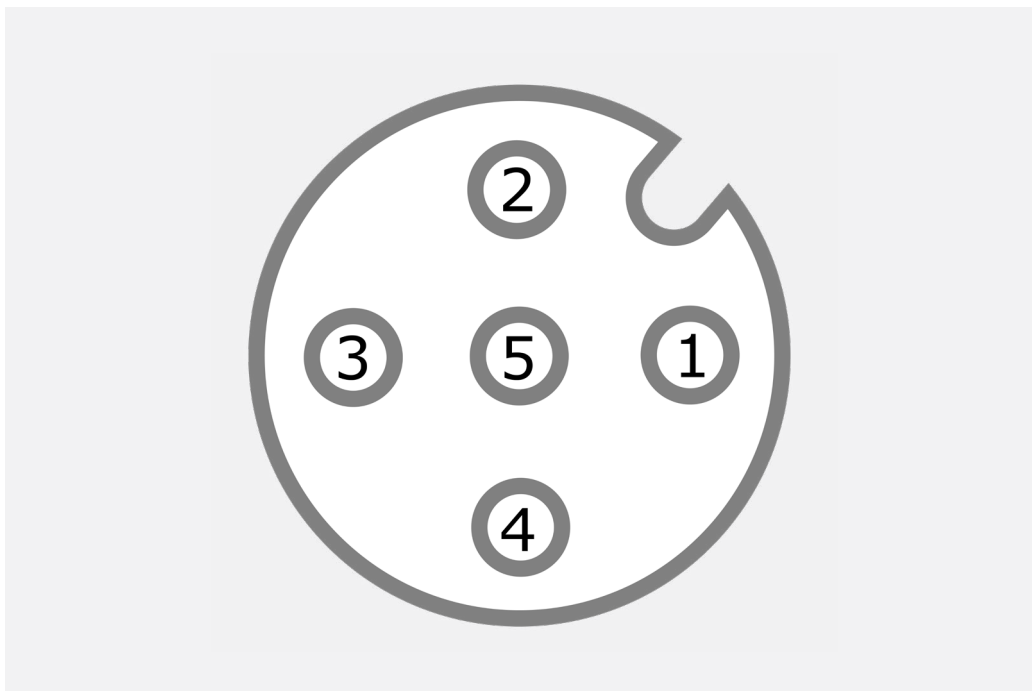
Figure 6.4.1 Connector layout of DR30, indicating PIN numbers (viewed from cable side).
