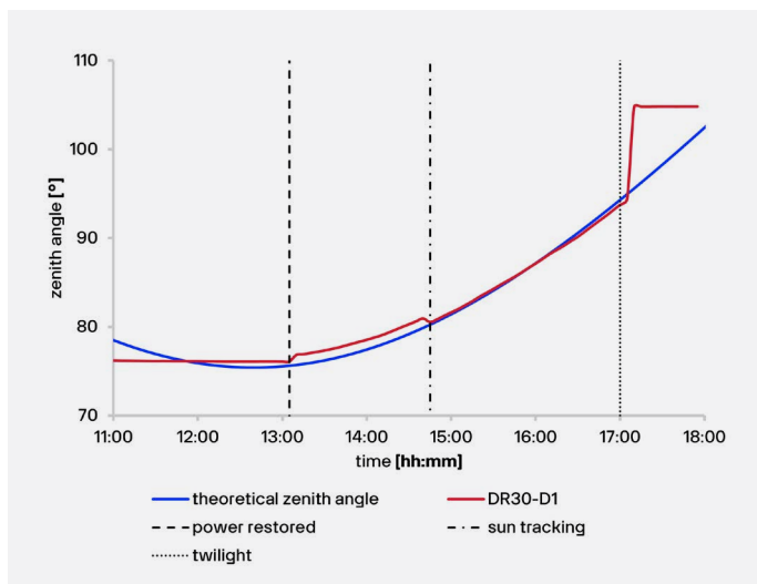
Figure 5.3.1 Example of use of the DR30 tilt sensor for tracker performance monitoring: the red line is the output of the DR30 tilt sensor, the blue line the theoretical zenith angle. There is a power failure before 13:00, at that time power is restored. Tracking between 13:00 and 15:00 is under cloudy conditions, based on GPS information only and slightly off. Tracking from 15:00 onwards is under sunny conditions and based on the tracker's sun sensor. The tracker moves to its rest position shortly after 17:00. Real measured data from Delft, the Netherlands.
