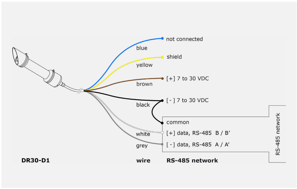
Figure 6.6.2 Connection of DR30 to an RS-485 network. DR30 is powered by an external power supply of 7 to 30 VDC.
